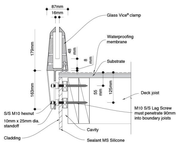
Architectural Bracket Detail for Cavity
