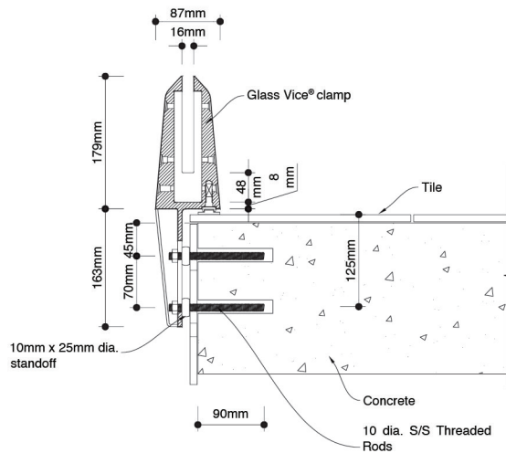
Architectural Bracket Detail for Concrete
