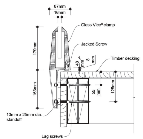
Architectural Bracket Detail for Decking
