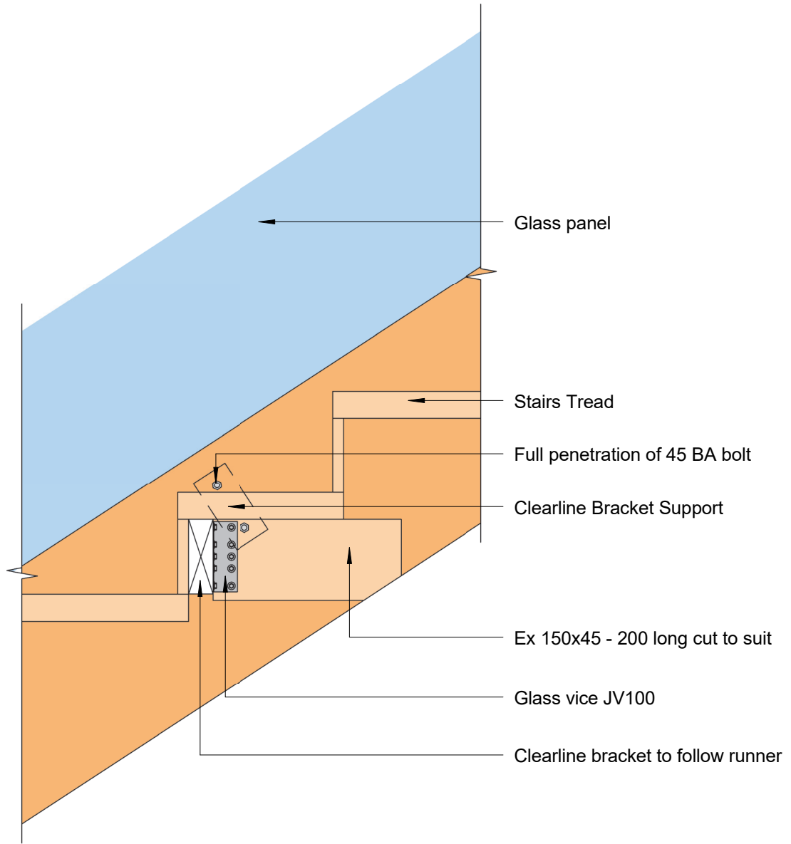
2 Section Detail View C-C 1 : 10
