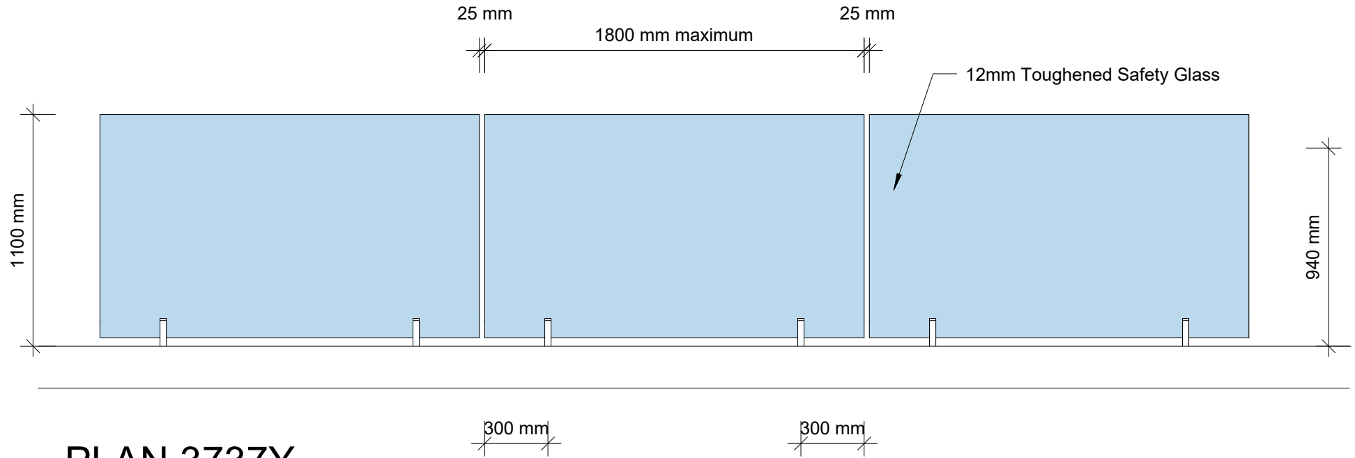
PLAN 3737Y
