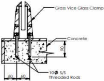
Top Fixed Detail
