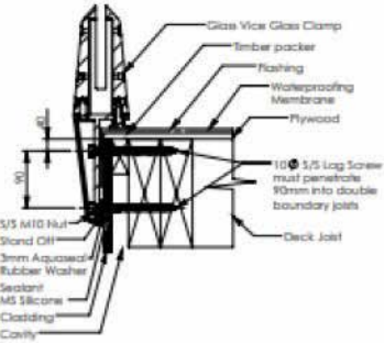
Side Fixed Detail
